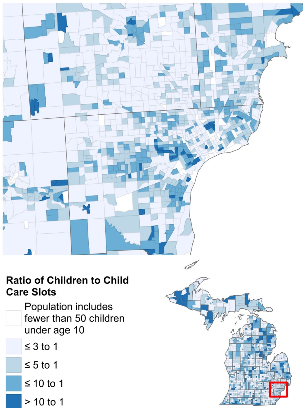
Figure 32. Ratio of Children Under Age 10 to Available Child Care Slots in Close Proximity, by Census Tract, Detroit
